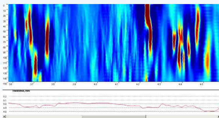
C-scan of the corrosion and trace of plate thickness
